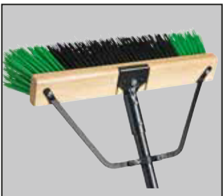
PB-700-GB18 - 18"/45cm PB-700-GB24 - 24"/60cm Ryno Push Broom - Medium Sweep Brace & Handle - Assembled
